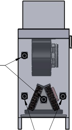
Option 1 Mounting (2) SLX-AAL-14 Locations
